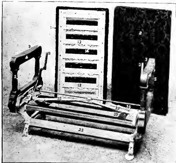
Fig. 3917. Sectional View.
